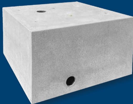
Grettir RAF - vörundur. S049 1.510 kg. 100x100x60 cm.
