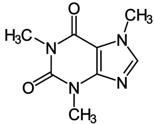
Caffeine (coffee)
